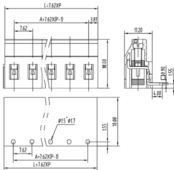
PCB Layout
