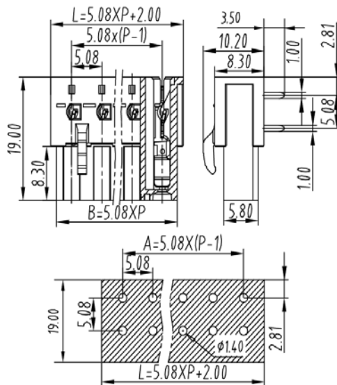
PCB Layout
